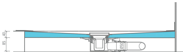
Channel drain, horizontal DN50 in timber
